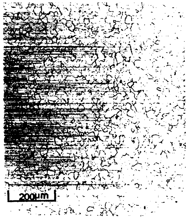
Fig. 8. Microstructure of 9.53-mm-thick tantalum plate as received from the mill.
